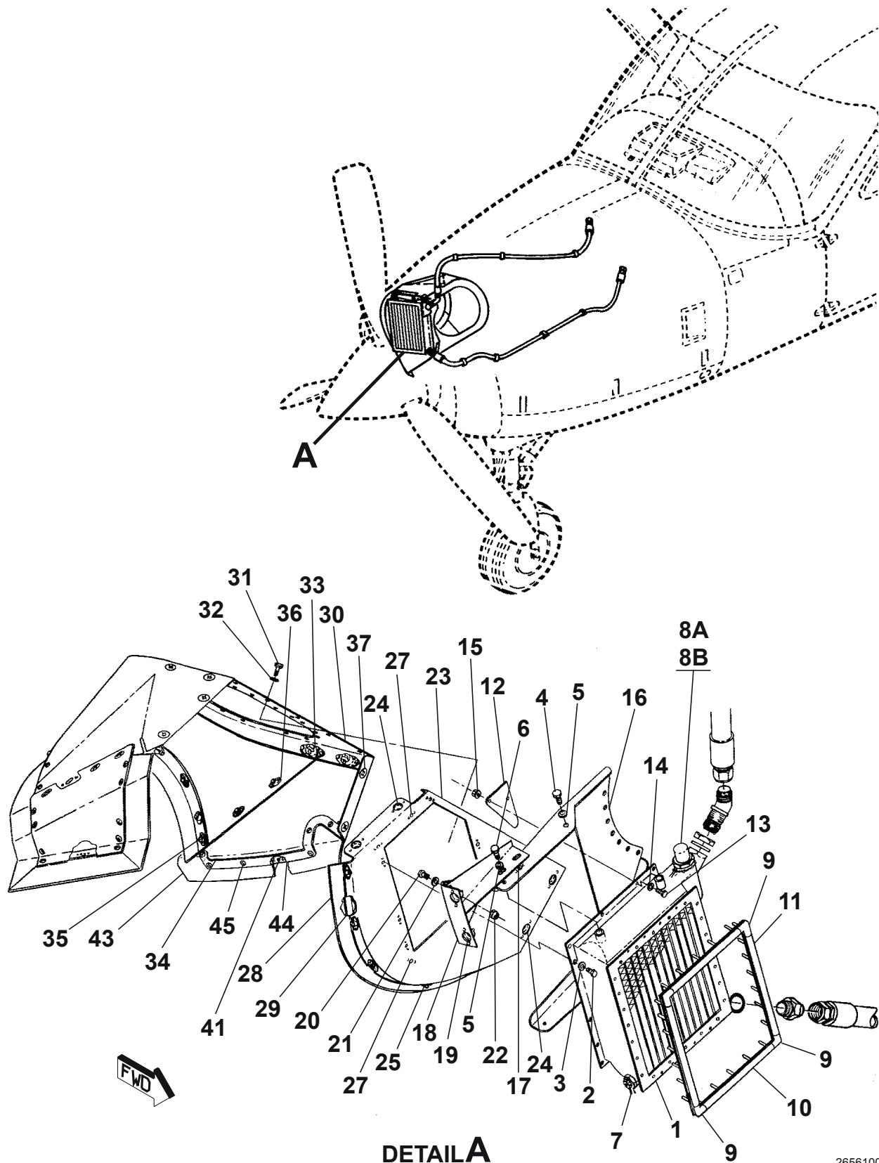
ENGINE OIL COOLING SYSTEM - SMALL Figure 01. (Sheet 1)
