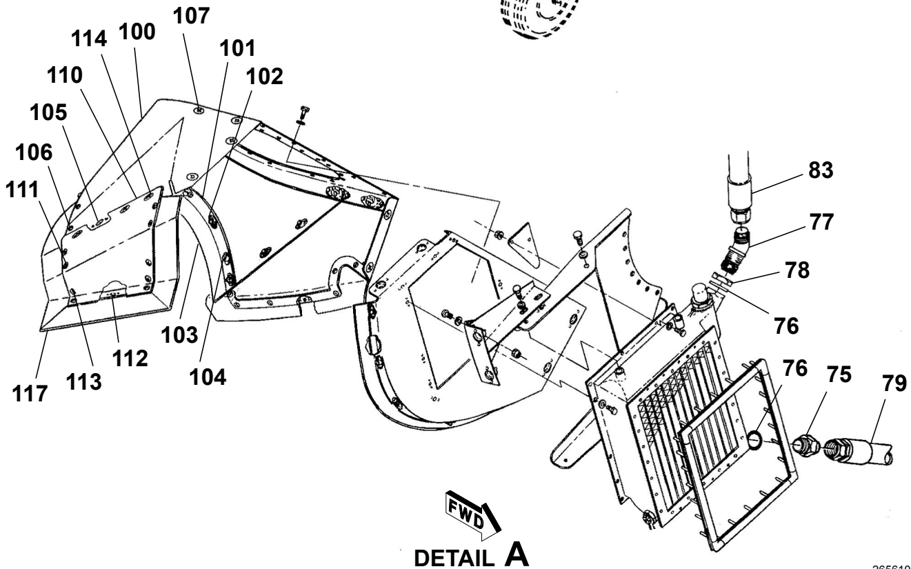
ENGINE OIL COOLING SYSTEM - SMALL Figure 01. (Sheet 2)
