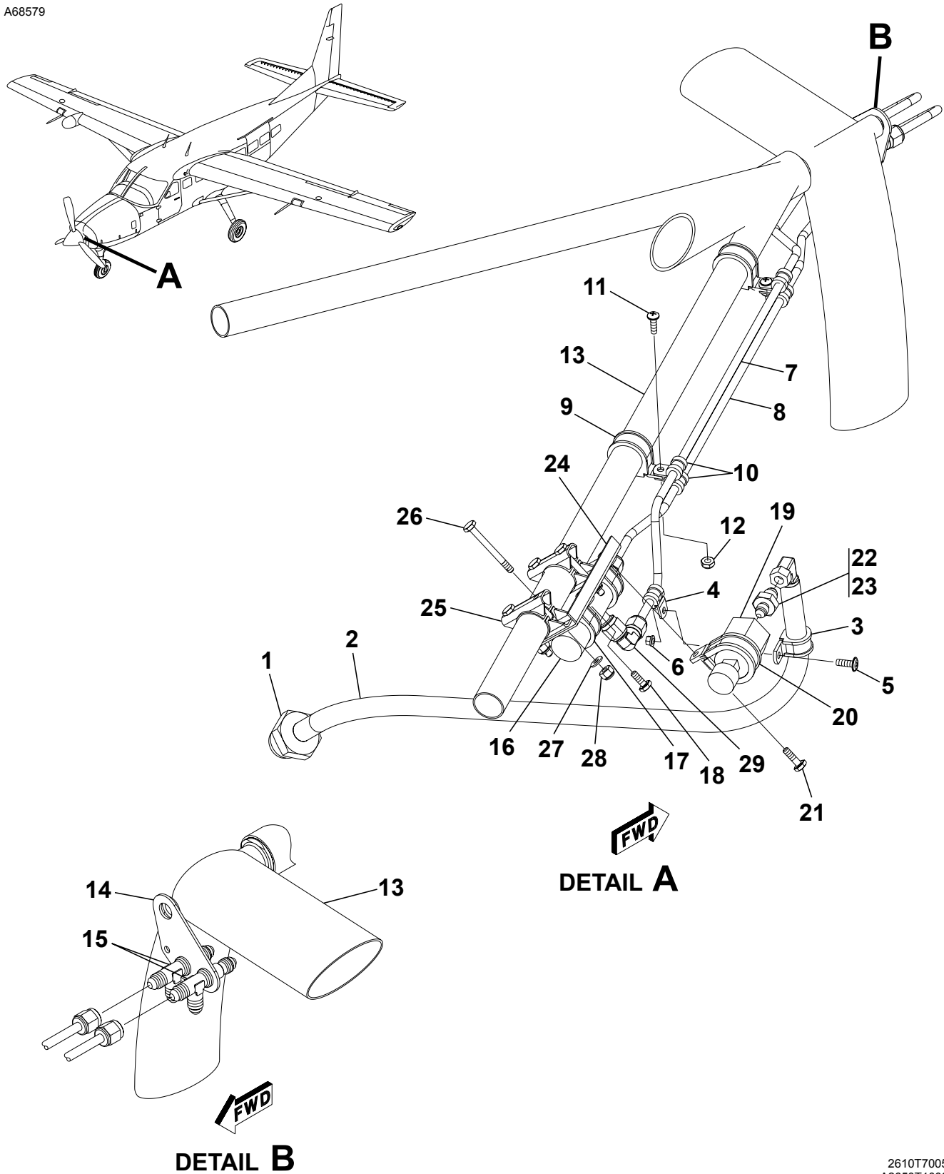
TKS OIL INDICATING Figure 02. (Sheet 1)
