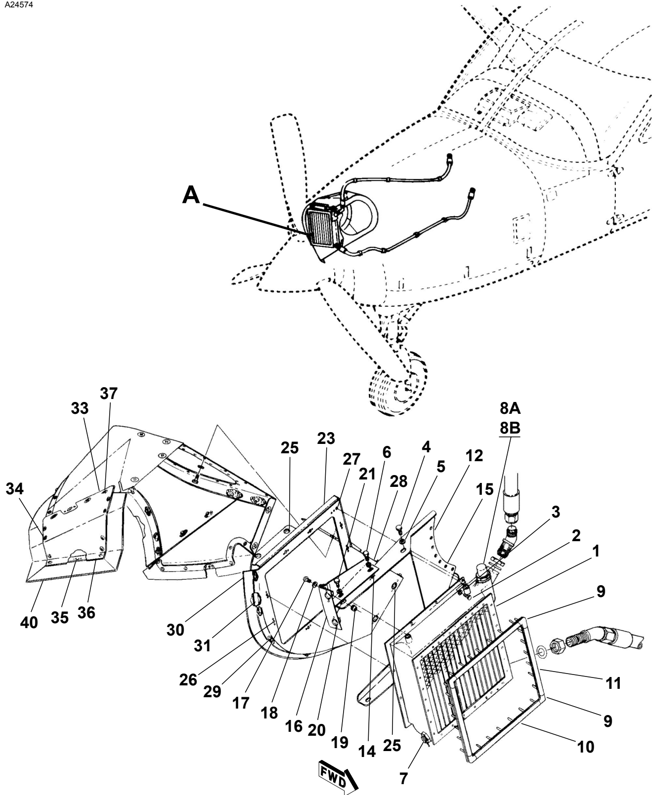
ENGINE OIL COOLING SYSTEM - LARGE Figure 02. (Sheet 1)
