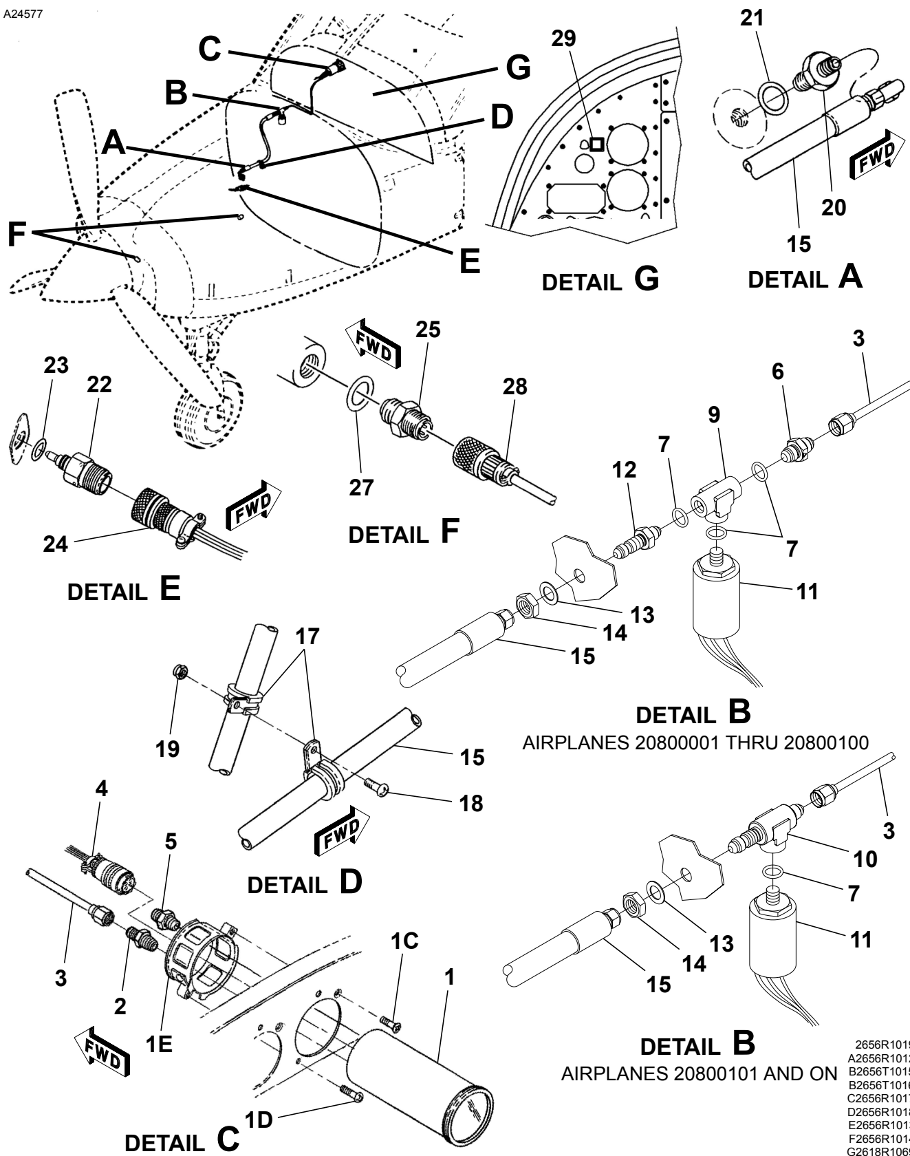
OIL INDICATING Figure 01. (Sheet 1)
