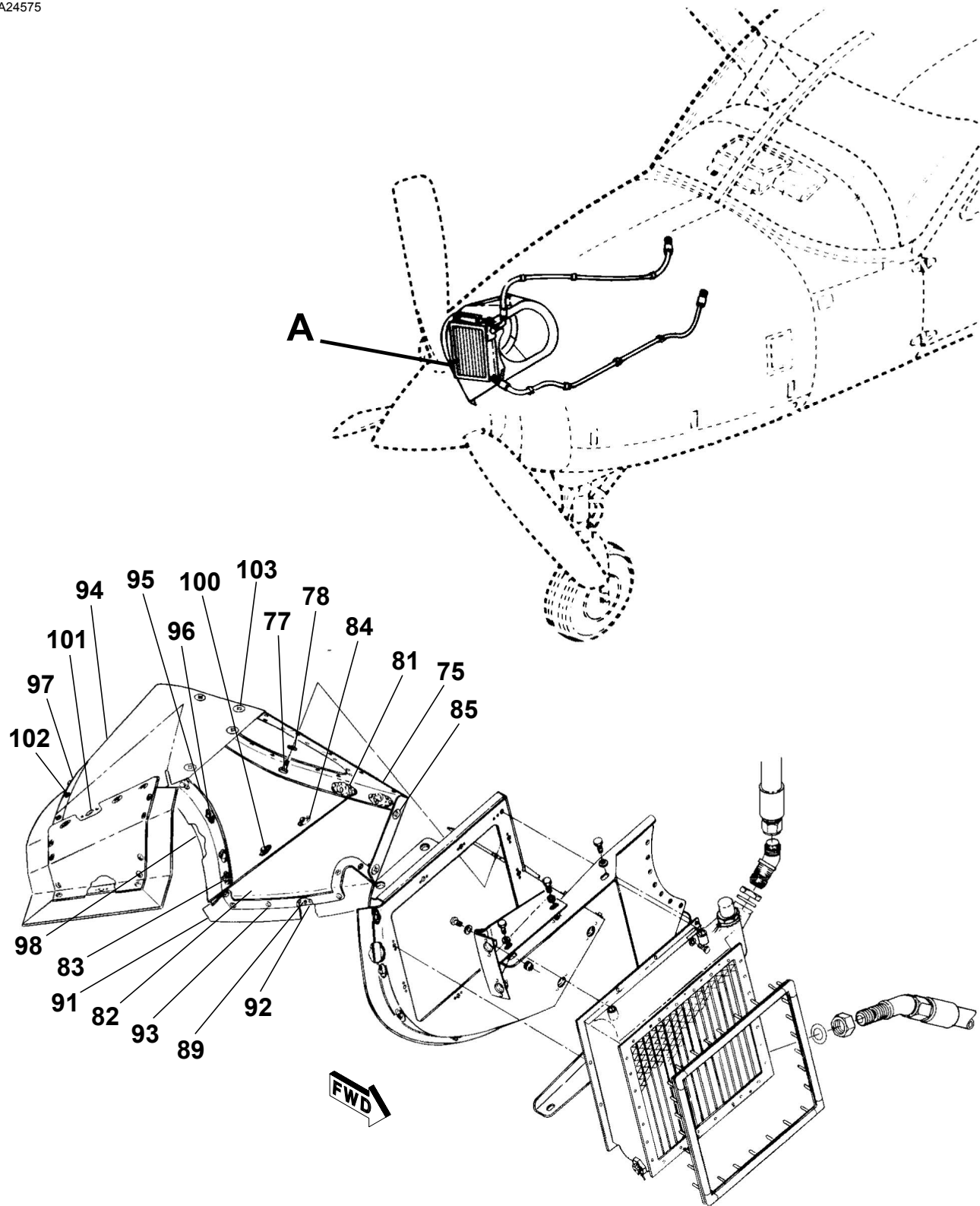
ENGINE OIL COOLING SYSTEM - LARGE Figure 02. (Sheet 2)
